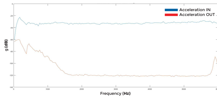
Accelerations - Modulus - Level 5 - 13 kg
